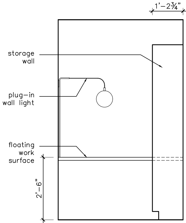
1 ELEVATION - FLEX DEN/OFFICE SCALE: 1/2" = 1'-0"
